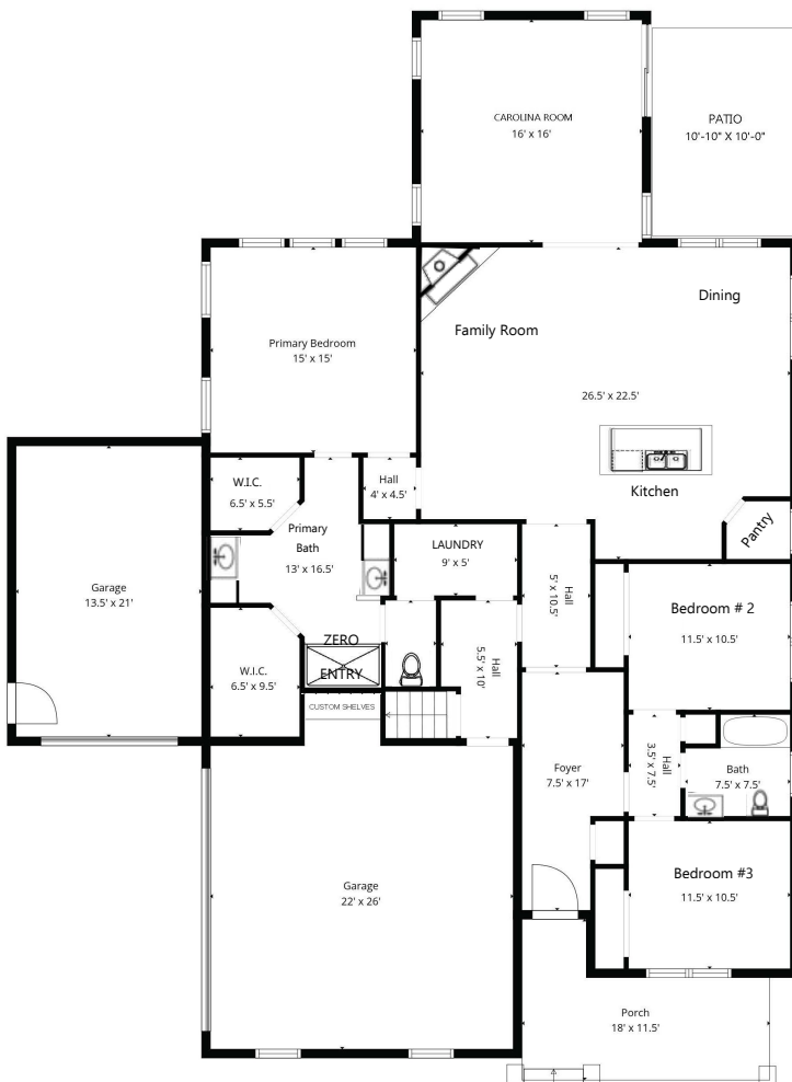
FIRST FLOOR
