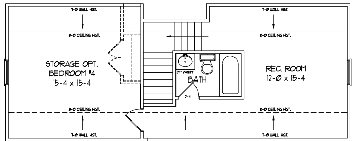
OPTIONAL SECOND FLOOR PLAN
