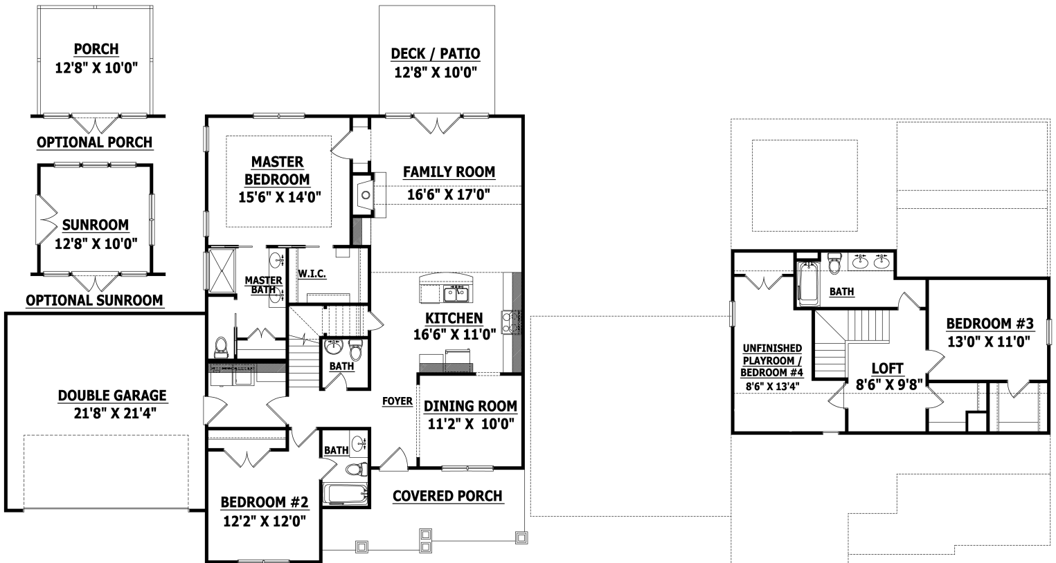
FIRST FLOOR
